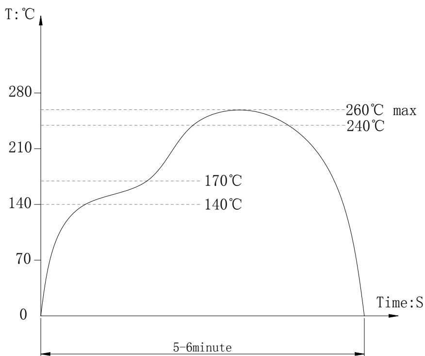
< Temperature profile >
